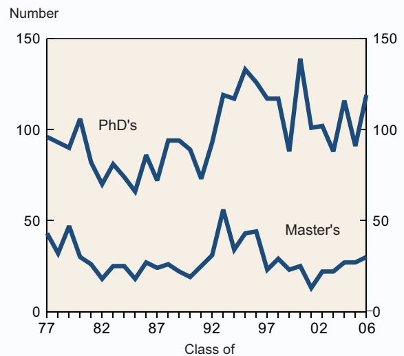
Figure 17. Astronomy master's degrees and doctorates awarded in the US, 1977-2006.
